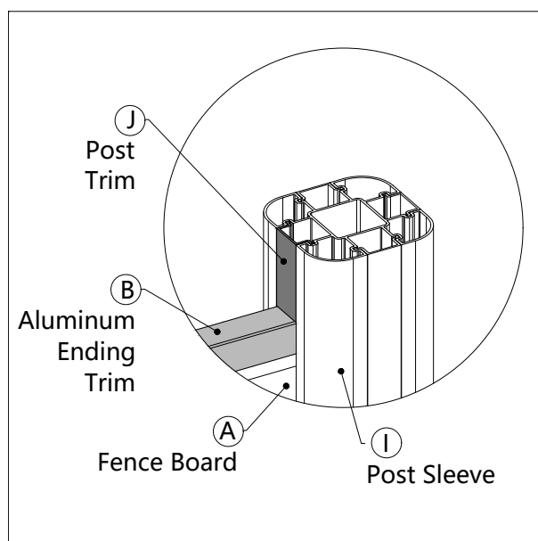
Detail 12-1
